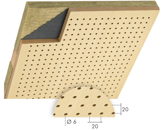
6 mm diameter hole 20 mm on center spacing
